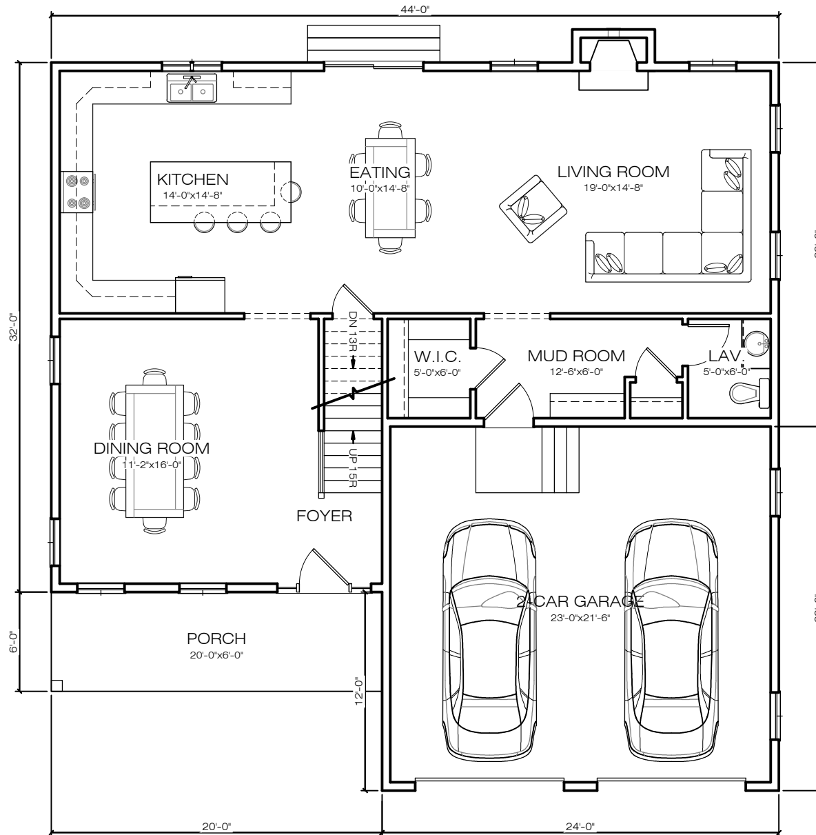
FIRST FLOOR PLAN 9'-0" CEILING HEIGHT 1,173 SQ. FT.
