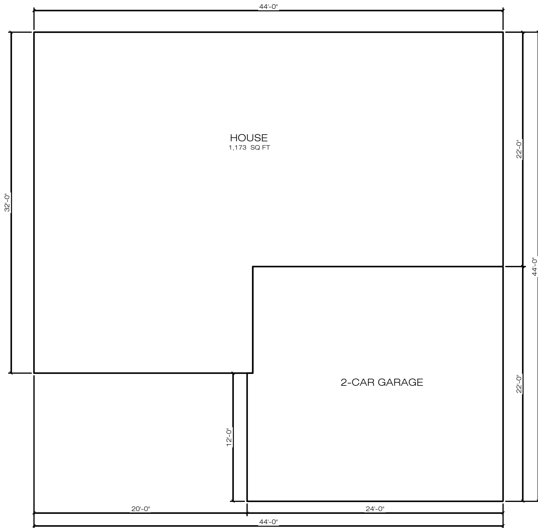
A BUILDING FOOTPRINT 1,173 SQ FT
